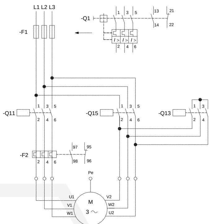
B) STAR-DELTA switching of three phase motor
